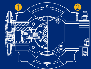
Twin Cylinder
